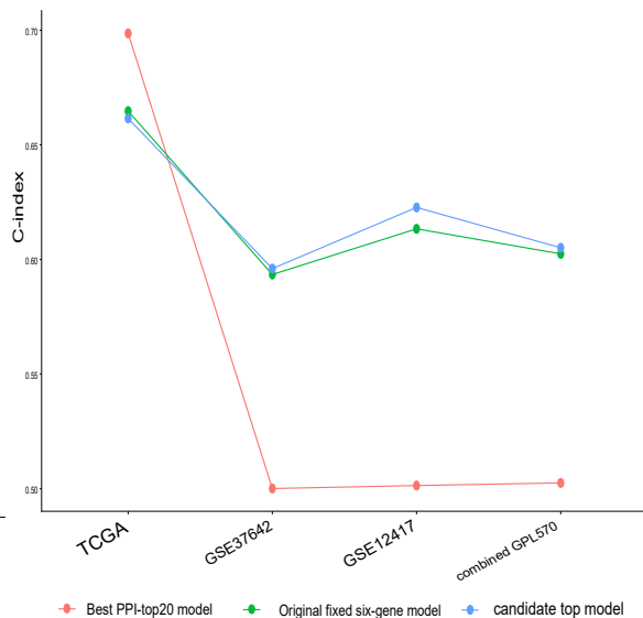
Original six-gene model versus candidate top model and best PPI-top20 model
