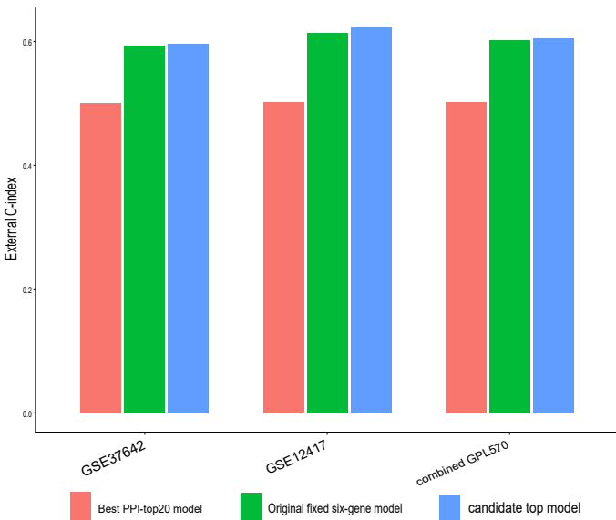
External validation comparison of fixed six-gene, candidate top, and best PPI-top20 model
